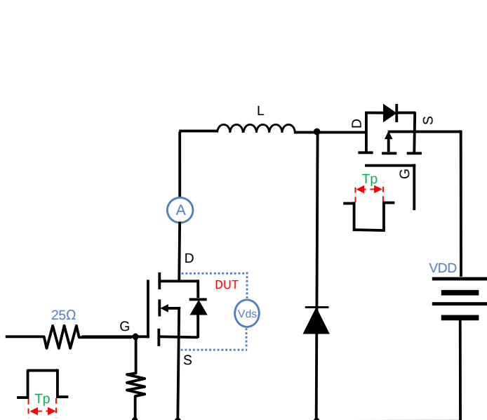
Figure A. Unclamped Inductive Switching (UIS) Test Circuit &amp; Waveform
