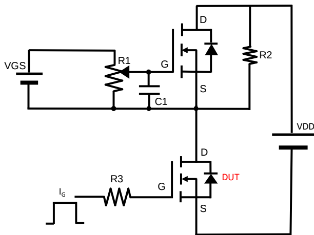
Figure B. Gate Charge Test Circuit &amp; Waveform
