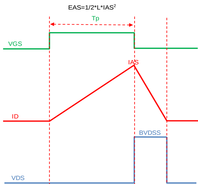
Figure A. Unclamped Inductive Switching (UIS) Test Circuit &amp; Waveform
